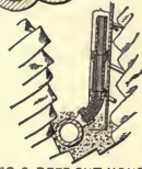
FIG. 9. DEEP-CUT HOUSE CONNECTION IN ROCK.
